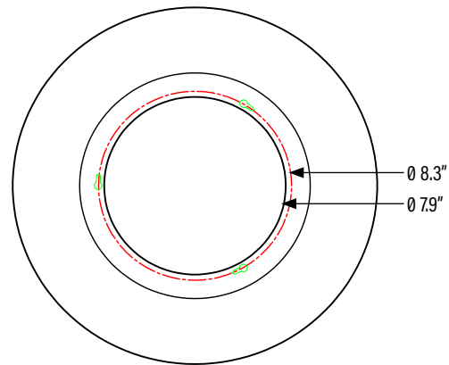
PARTS: 1 Aluminum Reflector + 3 Screws
